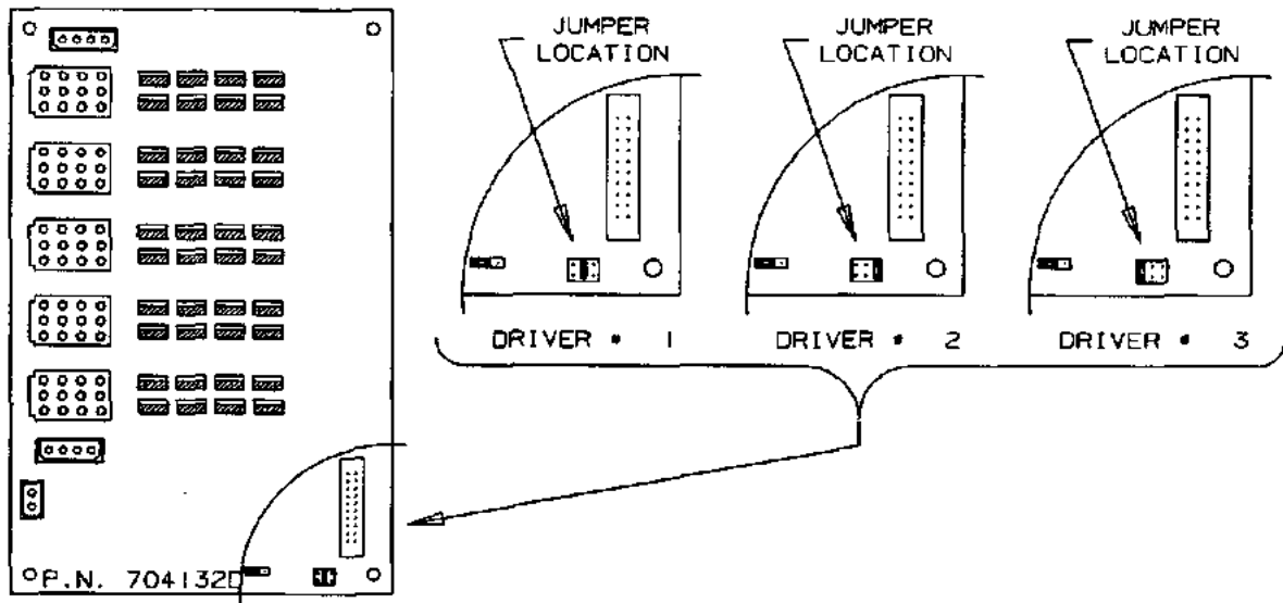
JUMPER LOCATION
